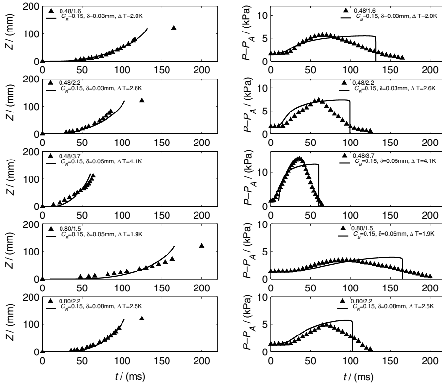
Fig. 8. Simulations with optimized parameters (Table 1).
