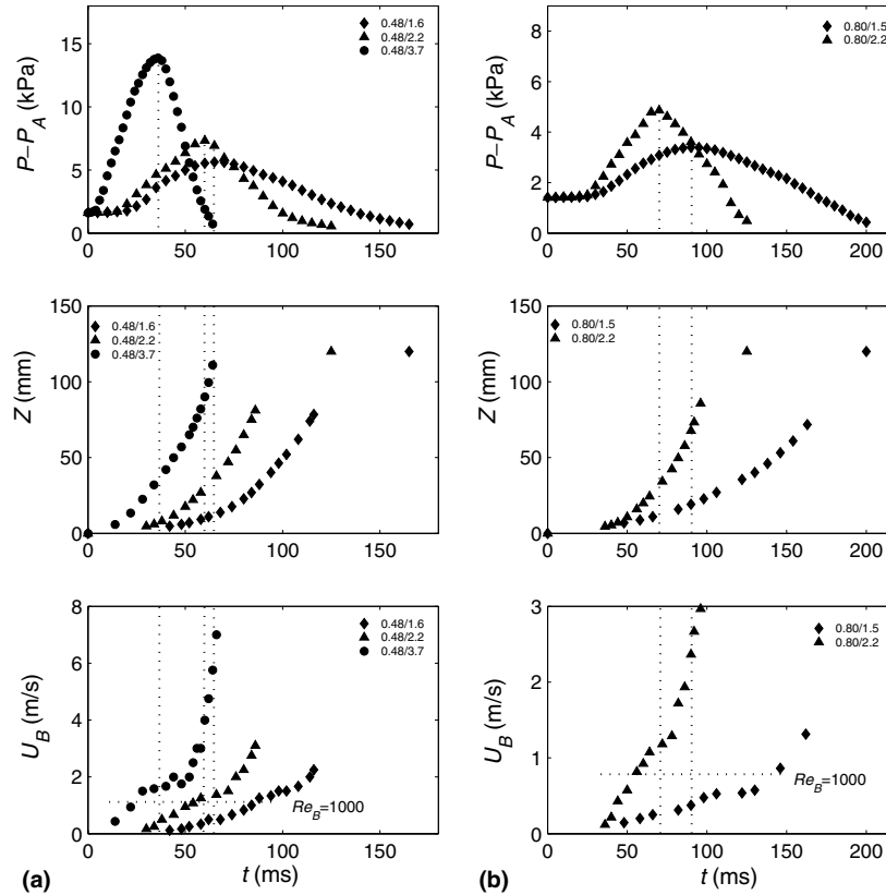
Fig. 3. Data for pressure P(t) - P_A , bubble length Z(t) and bubble velocity U_B(t) : (a) 0.48 mm tube; (b) 0.80 mm tube.
