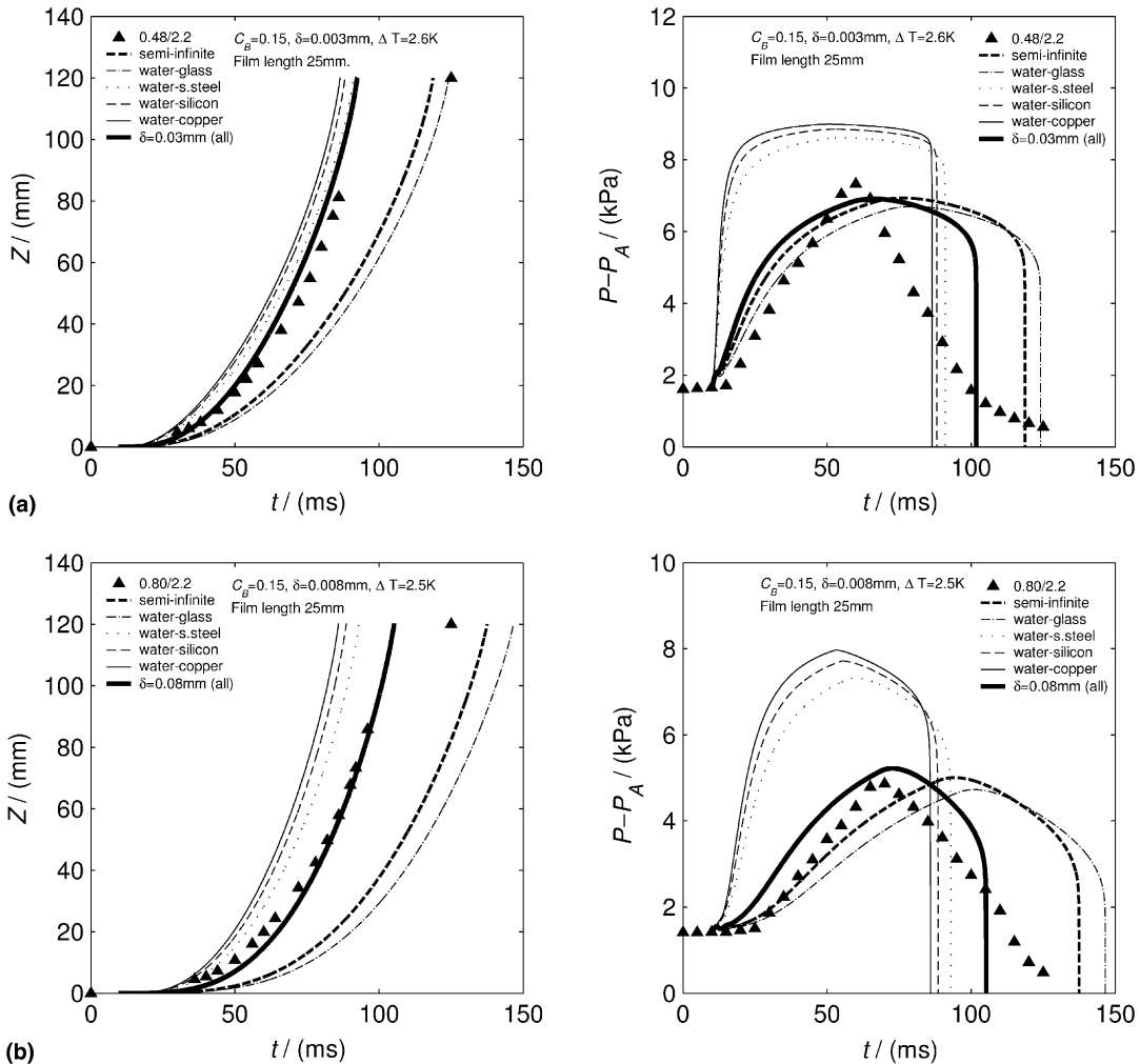
Fig. 14. Simulations with various wall materials and film roll-up with film length 25 mm: (a) 0.48 mm tube with \delta = 0.030 mm (optimized value, thick black line for all materials) and \delta = 0.003 mm; (b) 0.80 mm tube with \delta = 0.080 mm (optimized value, thick black line for all materials) and \delta = 0.008 mm.
