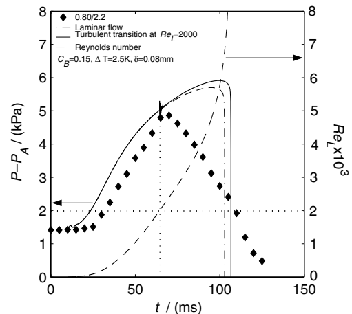
Fig. 9. Effect of laminar–turbulent transition on pressure pulse.
