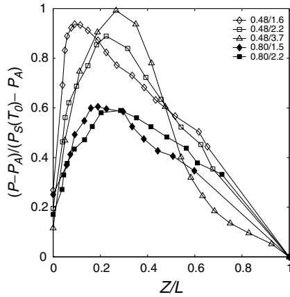
Fig. 5. Non-dimensional plot of pressure change versus bubble length for all runs.
