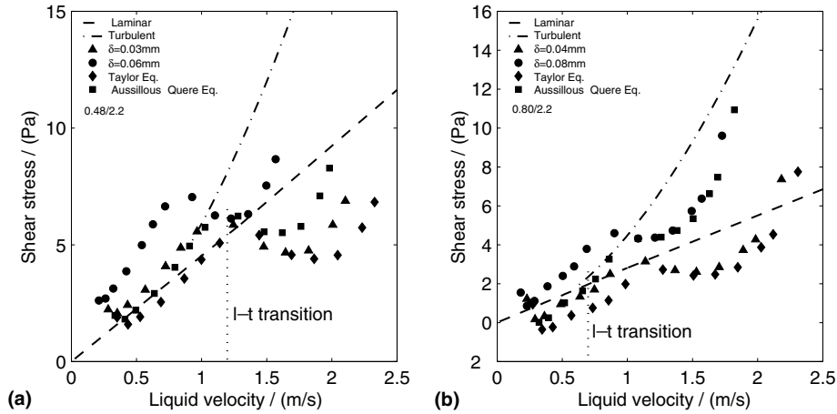
Fig. 11. Shear stress deduced from measured P(t) and Z(t) for different \delta(U_L) : (a) 0.48 mm tube; (b) 0.80 mm tube.
