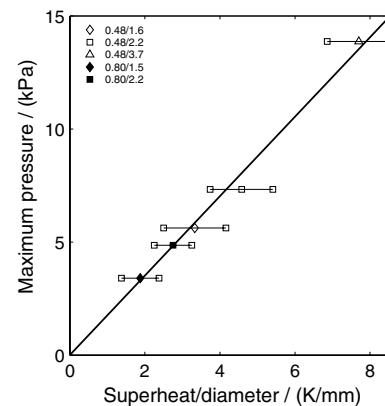
Fig. 4. Dependence of maximum pressure on initial superheat and tube diameter.
