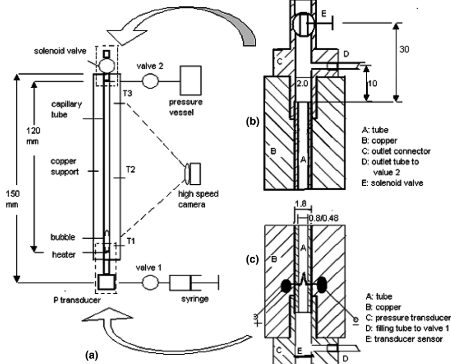
Fig. 1. Experimental apparatus.
