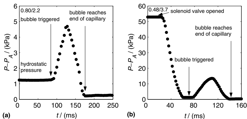
Fig. 2. Conditions prior to initiation of growth (a) without and (b) with prepressurization.
