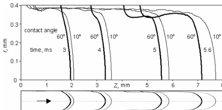
Fig. 10. Effect of dynamic contact angle on expulsion of liquid from an 8 mm long tube of diameter 0.8 mm by a constant gas pressure, Taha [27].
