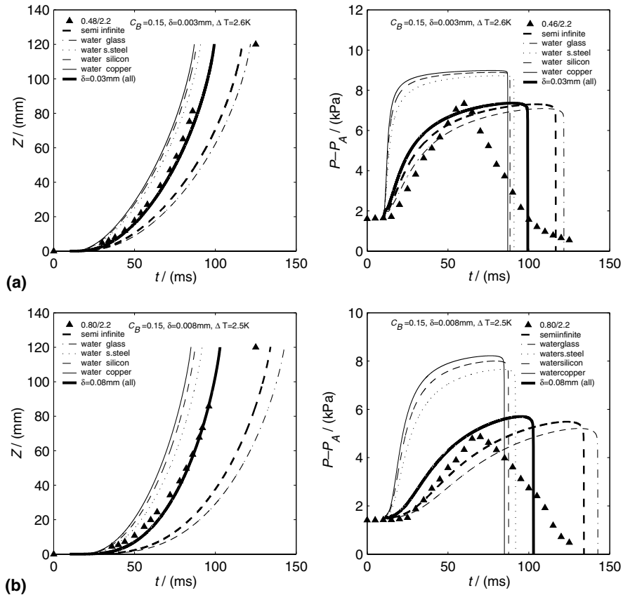
Fig. 12. Simulations with various wall materials: (a) 0.48 mm tube with \delta = 0.030 mm (optimized value, thick black line for all materials) and \delta = 0.003 mm; (b) 0.80 mm tube with \delta = 0.080 mm (optimized value, thick black line for all materials) and \delta = 0.008 mm.
