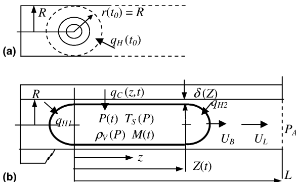
Fig. 6. Model for bubble growth.
