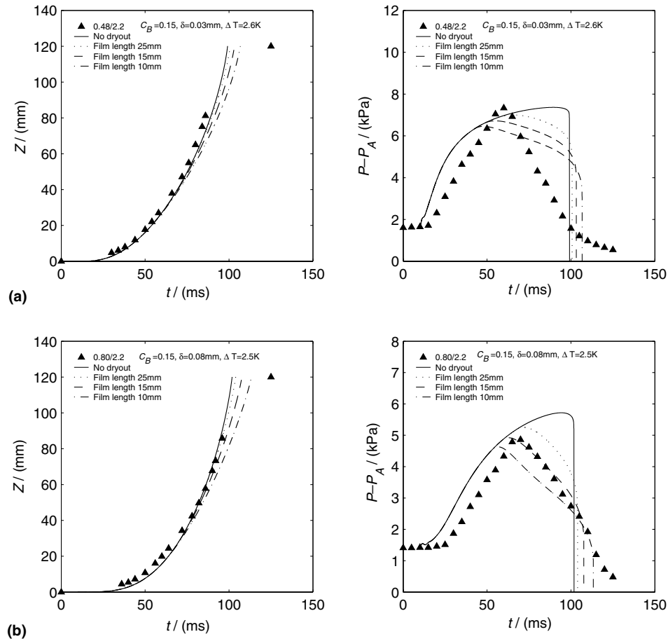
Fig. 13. Effect of simulated film roll-up with various film lengths: (a) 0.48 mm tube with optimized film thickness \delta = 0.030 mm; (b) 0.80 mm tube with optimized film thickness \delta = 0.080 mm.
